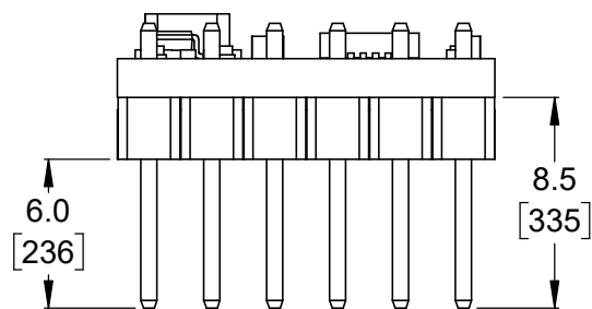
⑤ Profile with headers Scale 3:1
