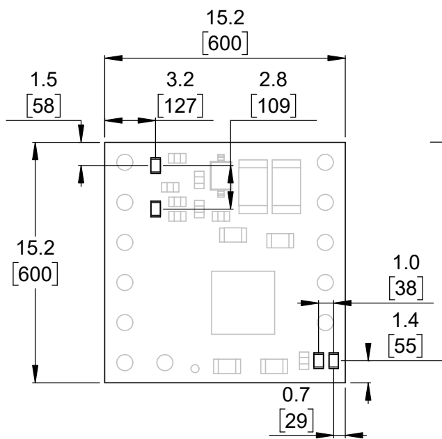
① Board dimensions (top view) Scale 3:1
