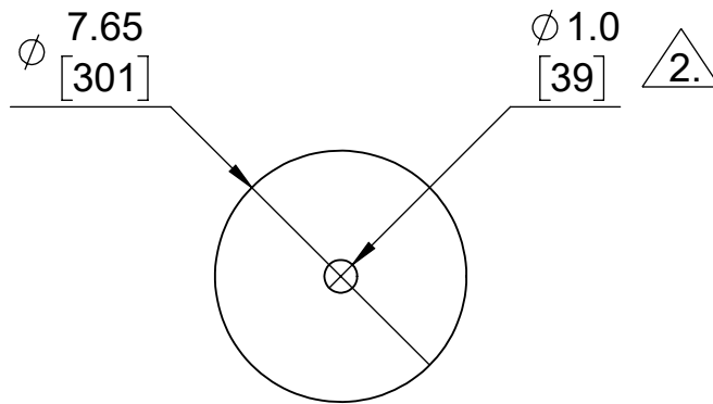
① Top view Scale 4:1
